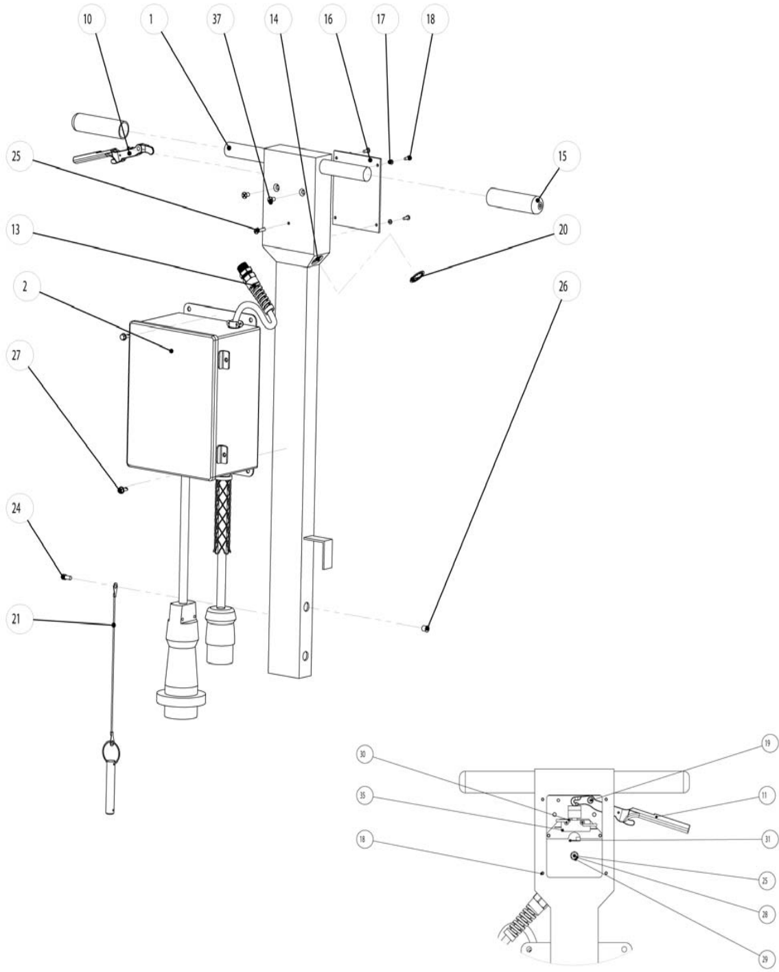
DETAIL A
