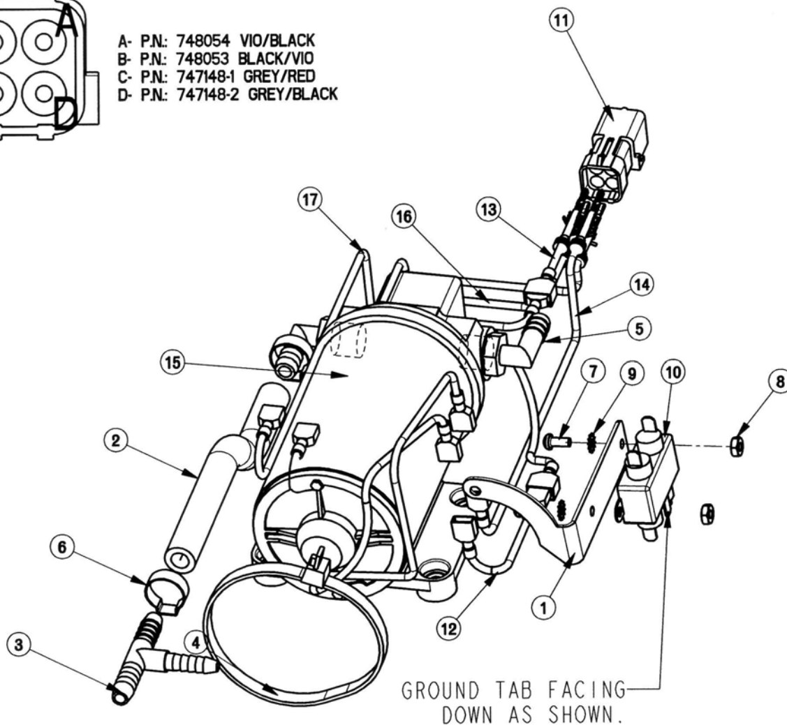
BILL OF MATERIAL - 742709-4
